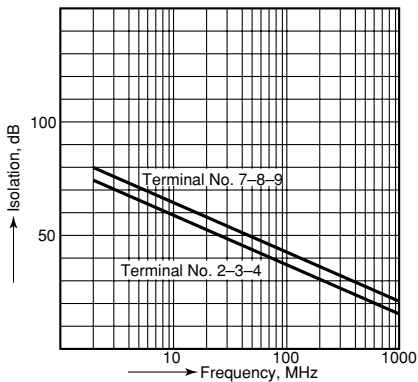
15-(1). High-frequency characteristics
