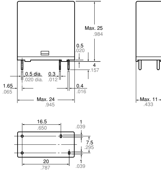
PC board pattern (Bottom view)
