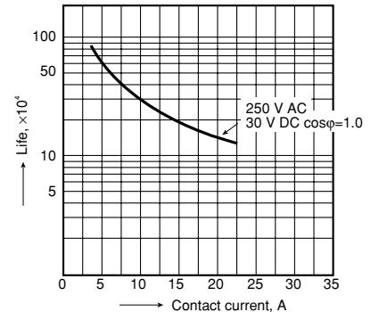
2. Life curve
