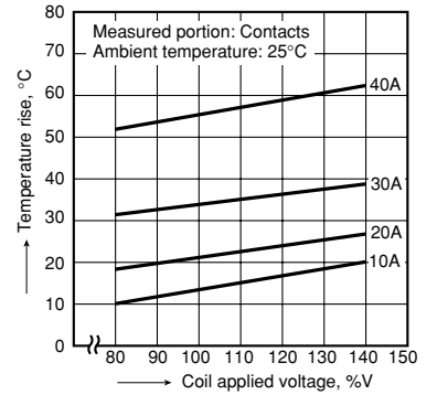
3.-1 Contact temperature rise (DC type)
