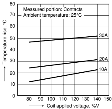
3.-1 Contact temperature rise (DC type)
