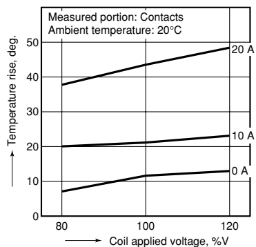
1. Contact temperature rise (DC type)
