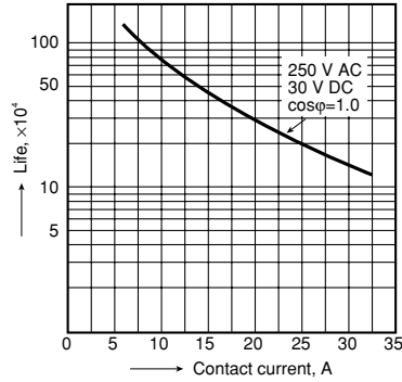
2. Life curve
