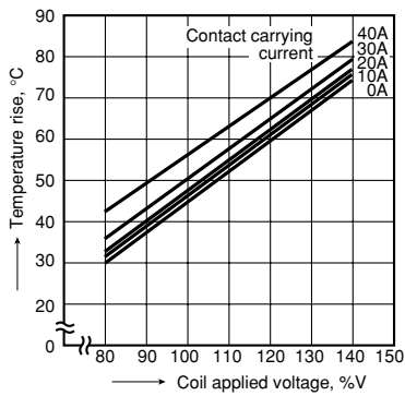
3.-2 Coil temperature rise (DC type)
