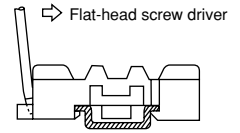
3. Removing from a DIN rail
