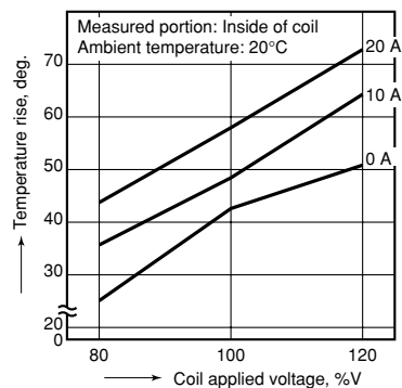
2. Coil temperature rise (DC type)
