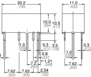
2 coil latching
