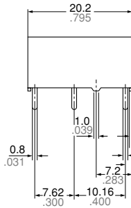
Single side stable 1 coil latching
