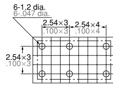
PC board pattern (Copper-side view) Single side stable 2 coil latching
