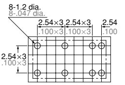
PC board pattern (Copper-side view) Single side stable 2 coil latching
